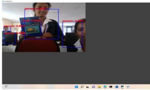
Figure 7: Objects Detection
