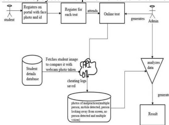
Figure 1: System Methodology
