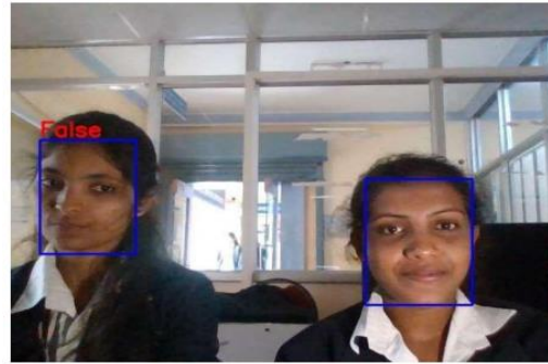
Figure 8: Face Spoofing
